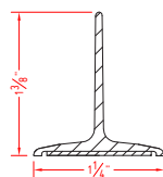
Cross Section Scale 1:1
