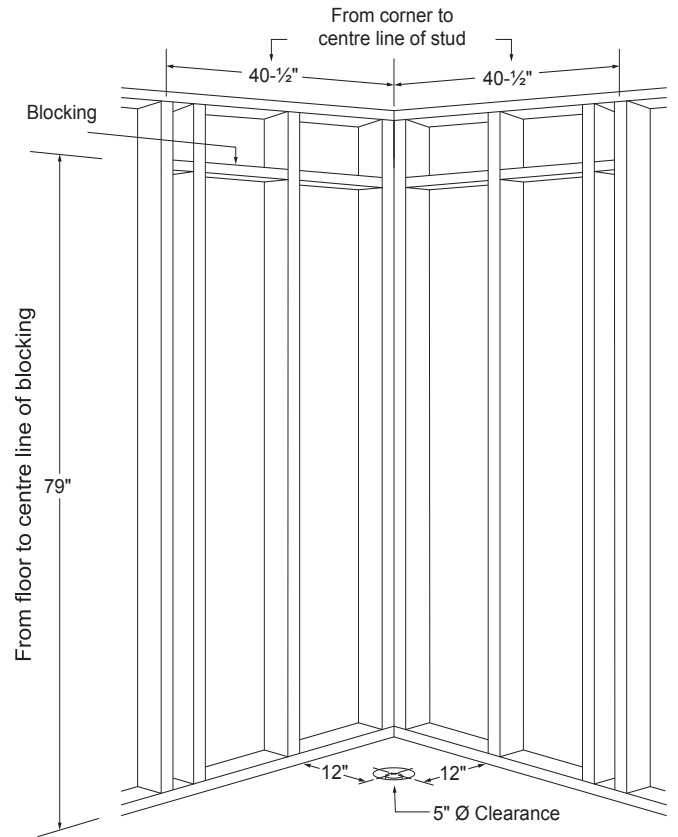
FIGURE 1 (2040NA/2042NA, 2040RF/2042RF)
